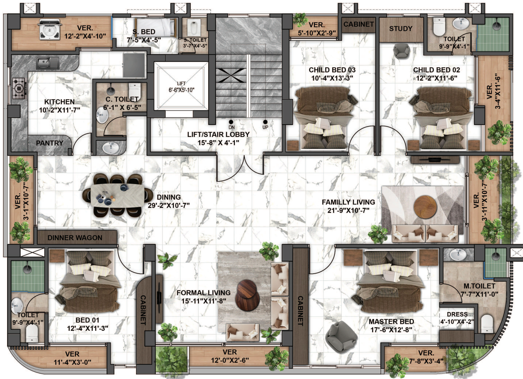
TYPICAL FLOOR PLAN
